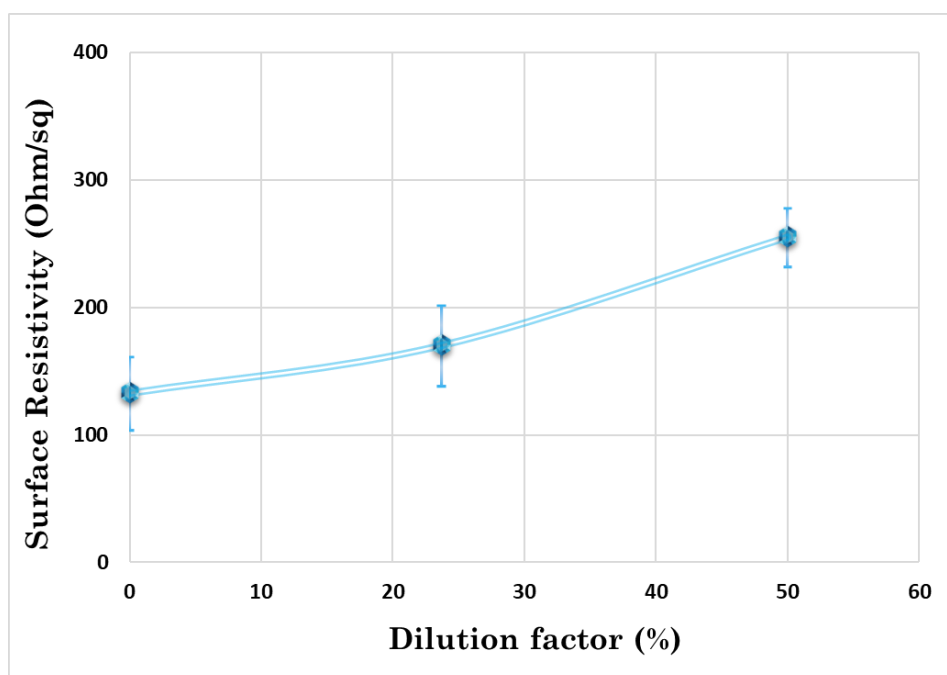
Figure 1. Surface resistivity of pure AQUACYL™ AQ0303 and the diluted aqueous mixtures
