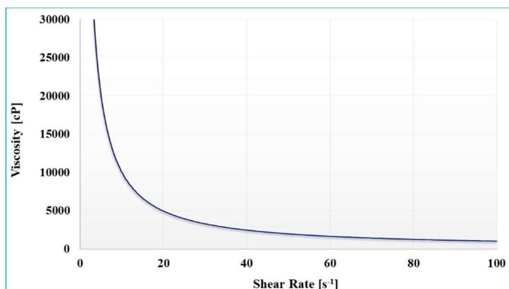
Figure 2. Viscosity flow curve of ORGACYL™ NMP0313 at 25°C
