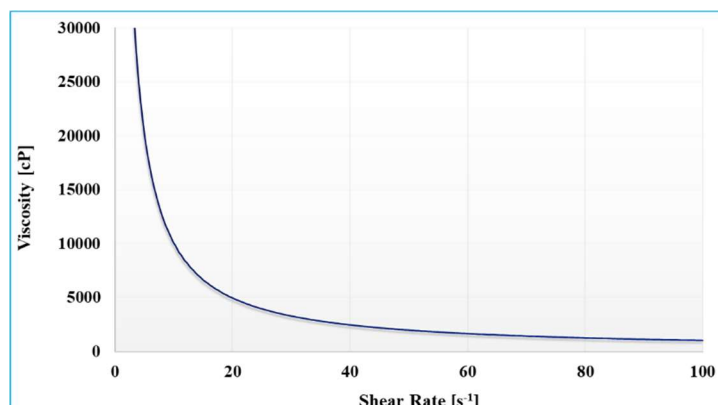
Figure 2. Viscosity flow curve of ORGACYL™ NMP2313 at 25°C
